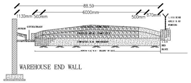
TYPE CROSS SECTION OF ROAD, APRRON, GUTTER/ DRAIN, WIRE FENCING COMPOUND
